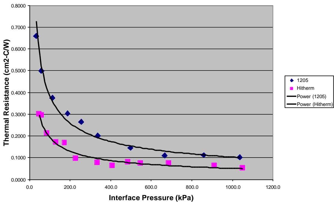
Variation of Thermal Resistance with Interface Pressure
